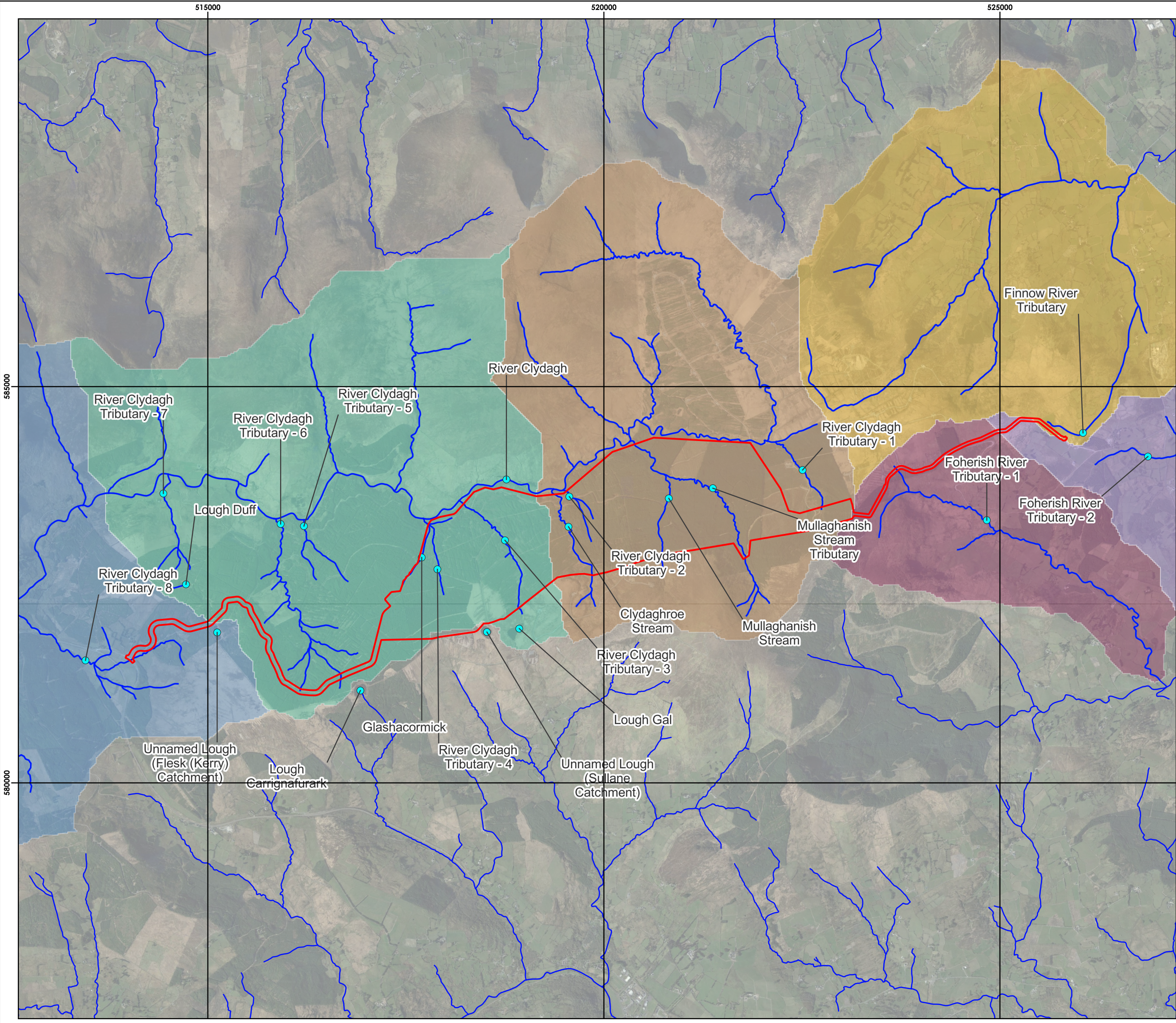
Figure 11-2 Internal Site Drainage
